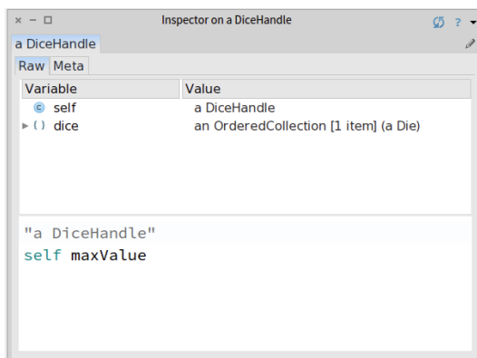
Figure 11-2 Inspecting and interacting with a die.
