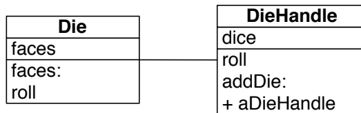
Figure 11-3 A die handle is composed of dice.
