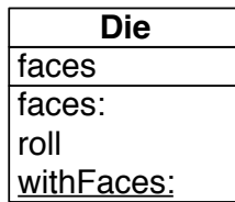
Figure 11-1 A single class with a couple of messages. Note that the method withFaces: is a class method.
