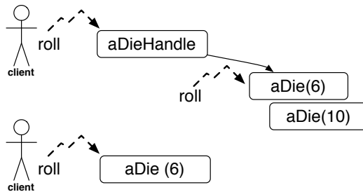
Figure 11-7 A polymorphic API supports the Don't ask, tell principle.
